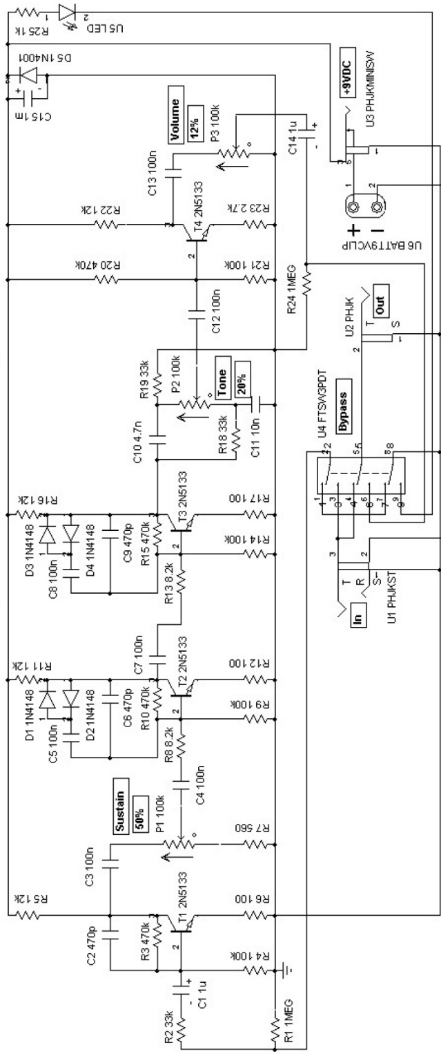
Big Muff 1Pi Effect Schematic
