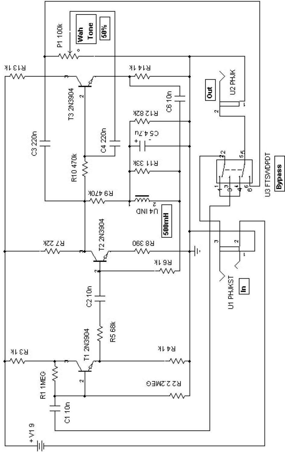
Wah Tone Effect Schematic
