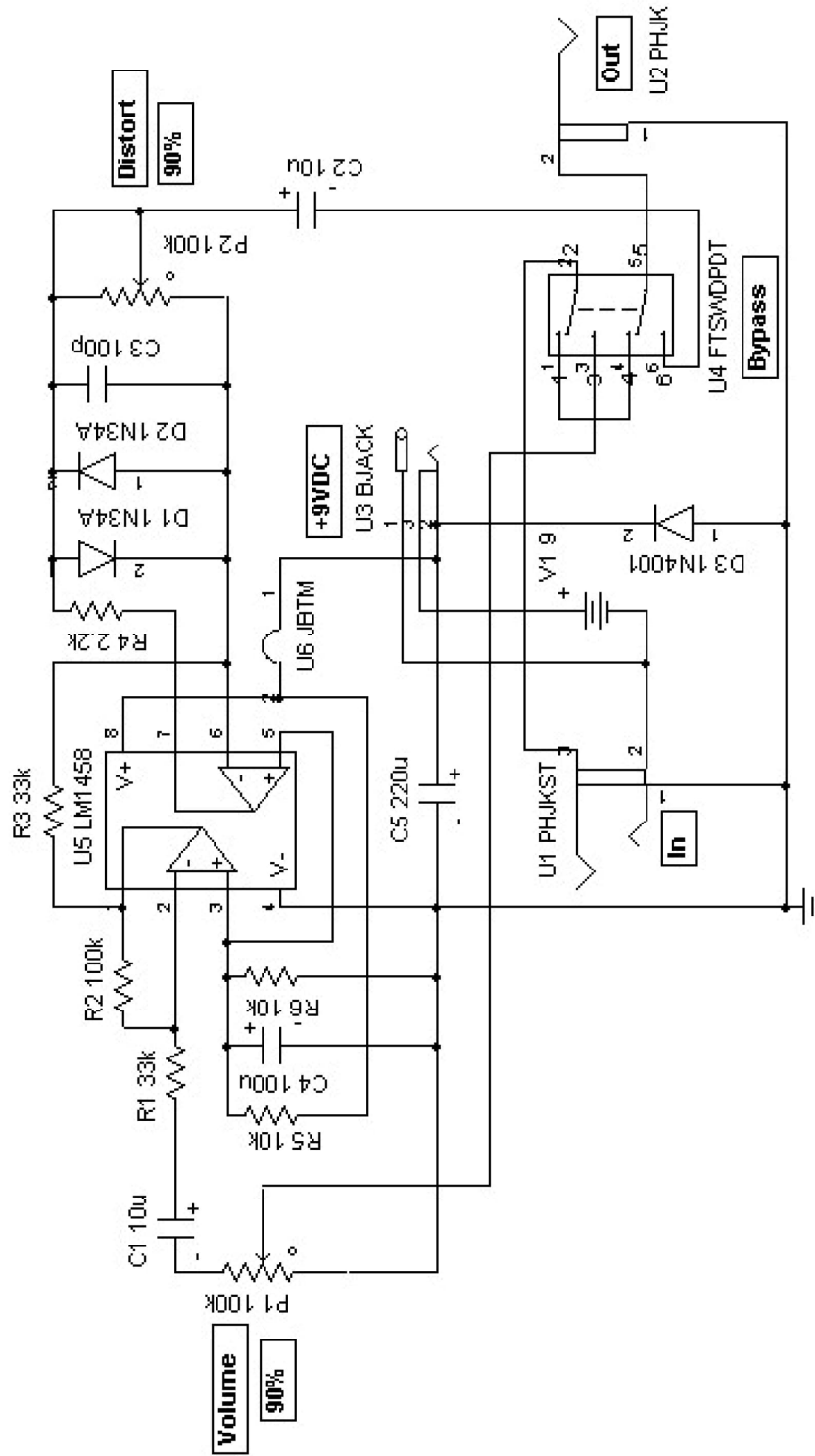
Electric Guitar Distortion Effect Schematic
