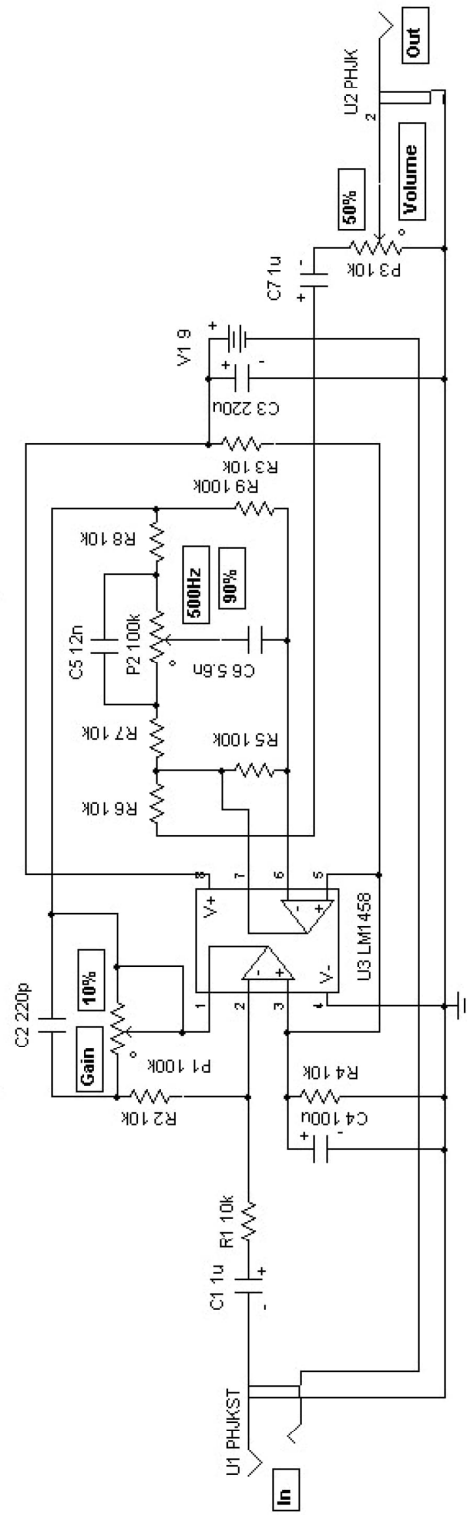
LM1458 1 Band Equalizer Schematic
