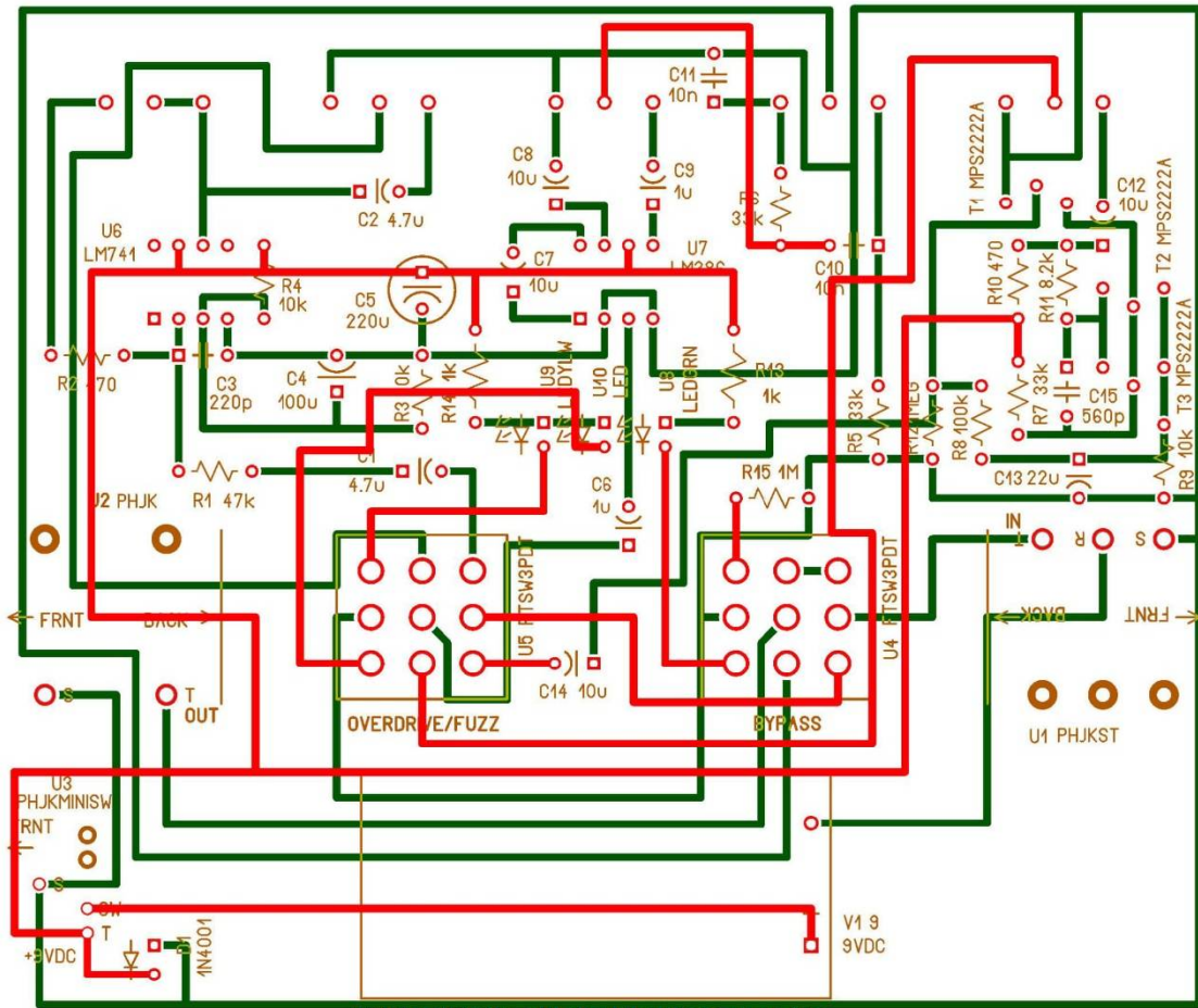
LM741-LM386 OVERDRIVE/FUZZ EFFECT
