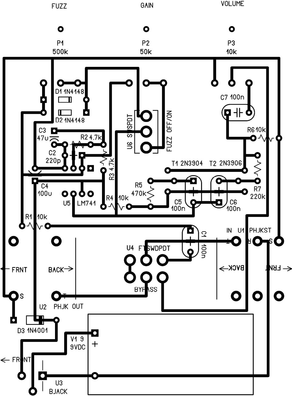
LM741/TRANSISTORS OCTAVE FUZZ EFFECT
